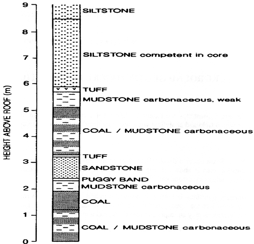
Fig. 2 - Elouera Colliery Geological profile - Thompson Panel
