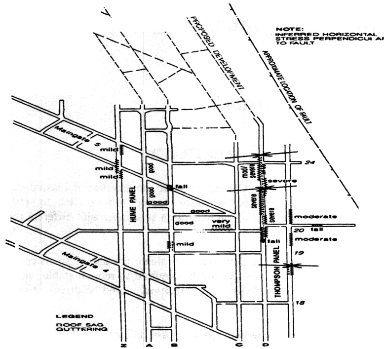
Fig. 1 - Elouera Colliery panel layout roadway deformation, layout and inferred stress direction
