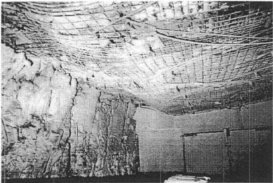
7(a) Leading roadway D heading, outbye 24 line, Thompson Panel
